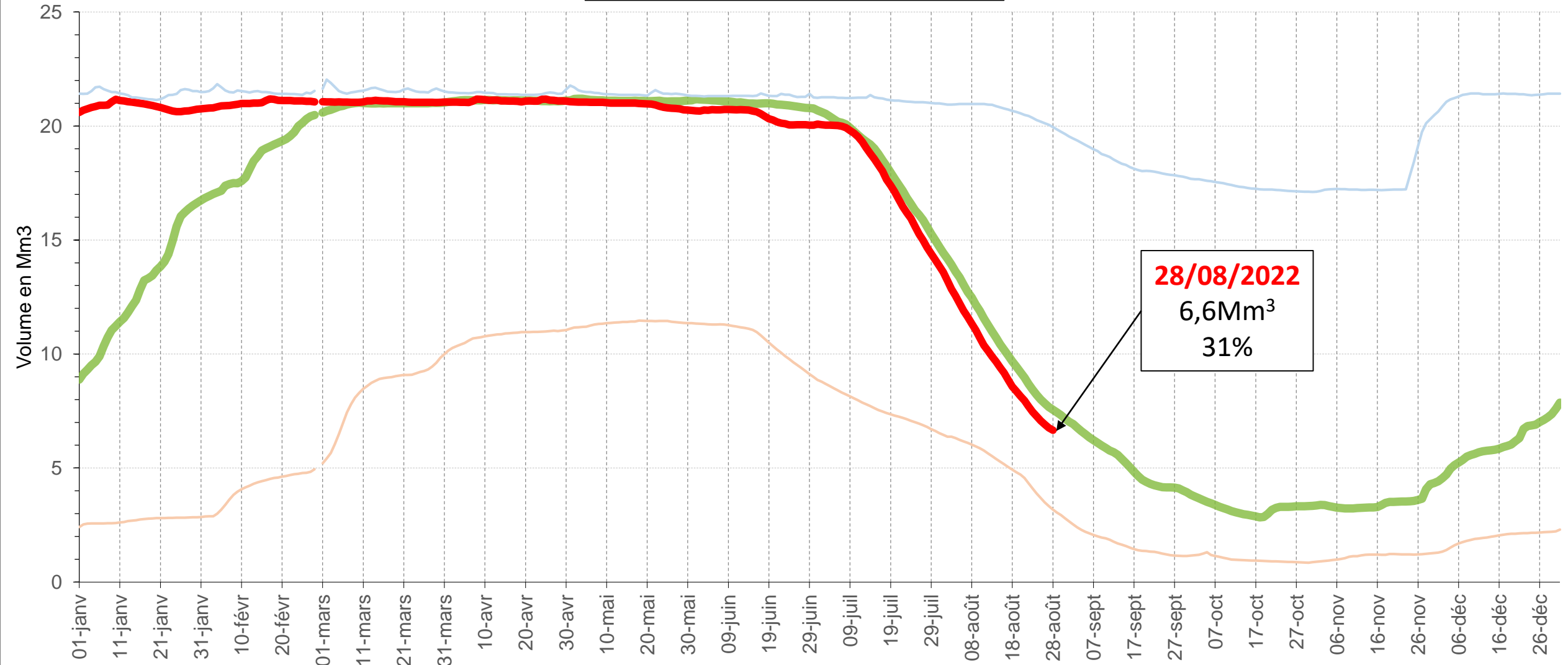
Volume Lavaud - Mas Chaban (2000-2022)
